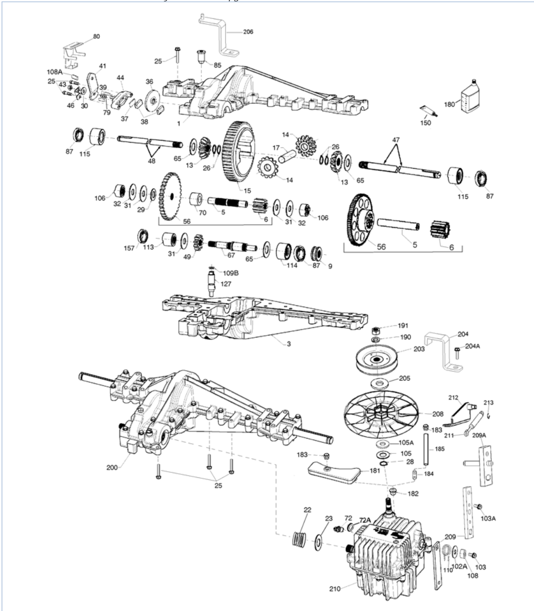
lth2000 2000-2000-004D / Hydro Transaxle pg 1
